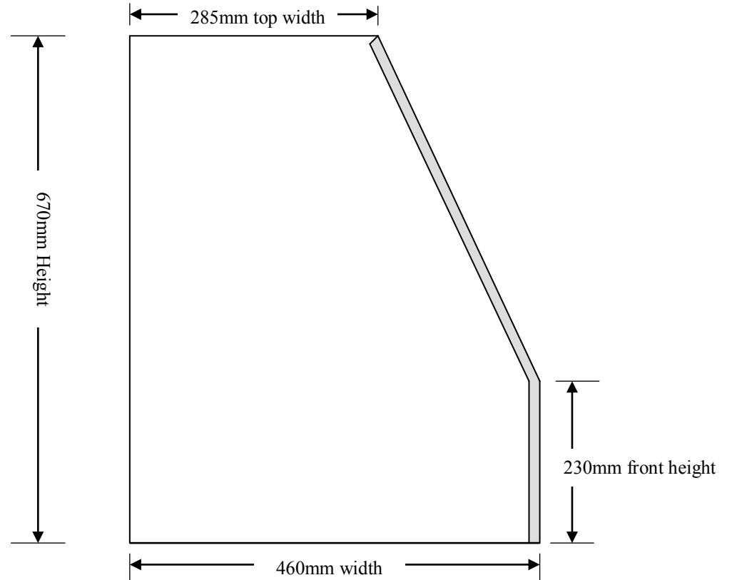
Side View
